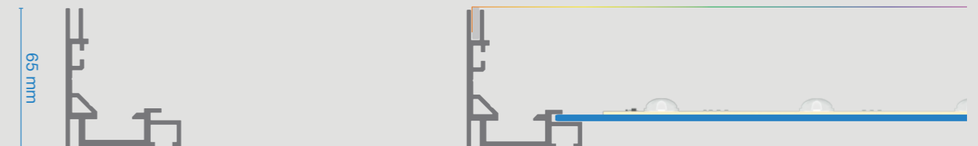
Profildesign mf-65 / profile design mf-65
